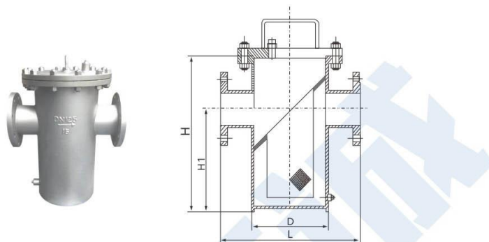
篮式过滤器安装尺寸 Basket filter installation size
